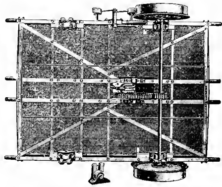
Fig. 5582. View of Underside, showing Roller Bearings.
